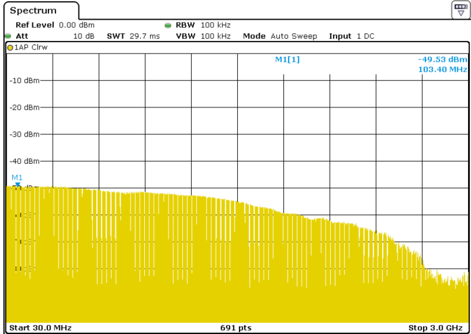
Figure 1 – 5 MHz comb frequency; amplifier off
